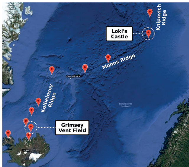
Fig. 1: Arctic Mid-Oceanic Ridge (AMOR) with the two proposed working areas Grimsey Vent Field (GVF) and Loki's Castle as well as additional vent fields (Beaulieu, 2015).
